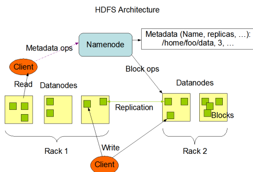
Figure 4 Architecture de HDFS
